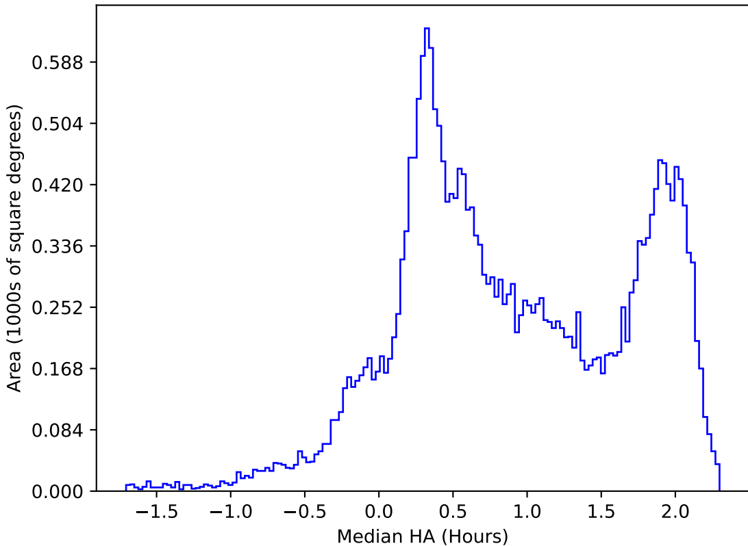
too_elab_r32_d2_ugrizy_v3.4_10yrs All sky all bands: Median HA
