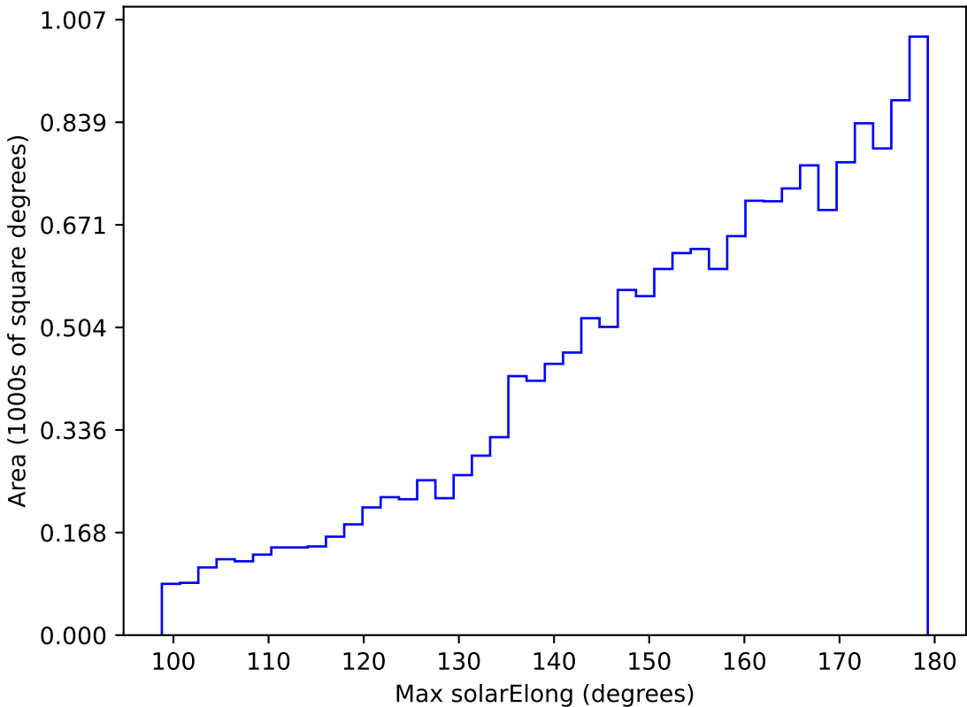
too_elab_r32_d2_ugrizy_v3.4_10yrs WFD y band: Max solarElong
