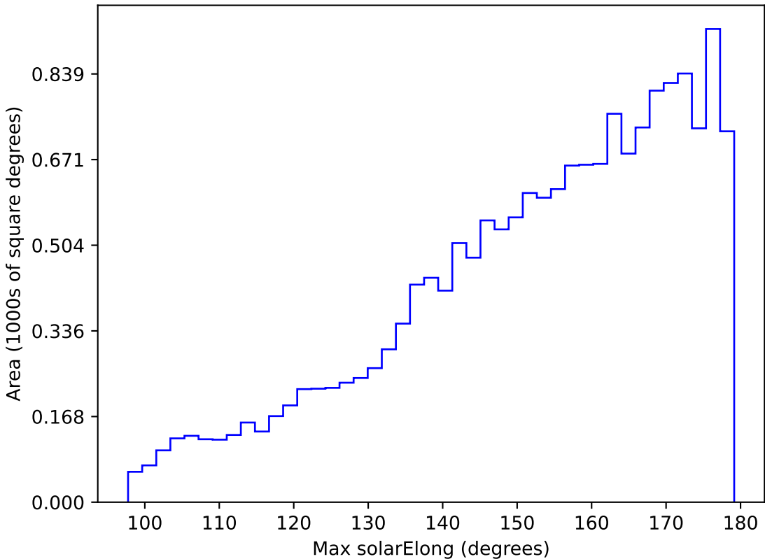
too_elab_r32_d2_ugrizy_v3.4_10yrs WFD u band: Max solarElong
