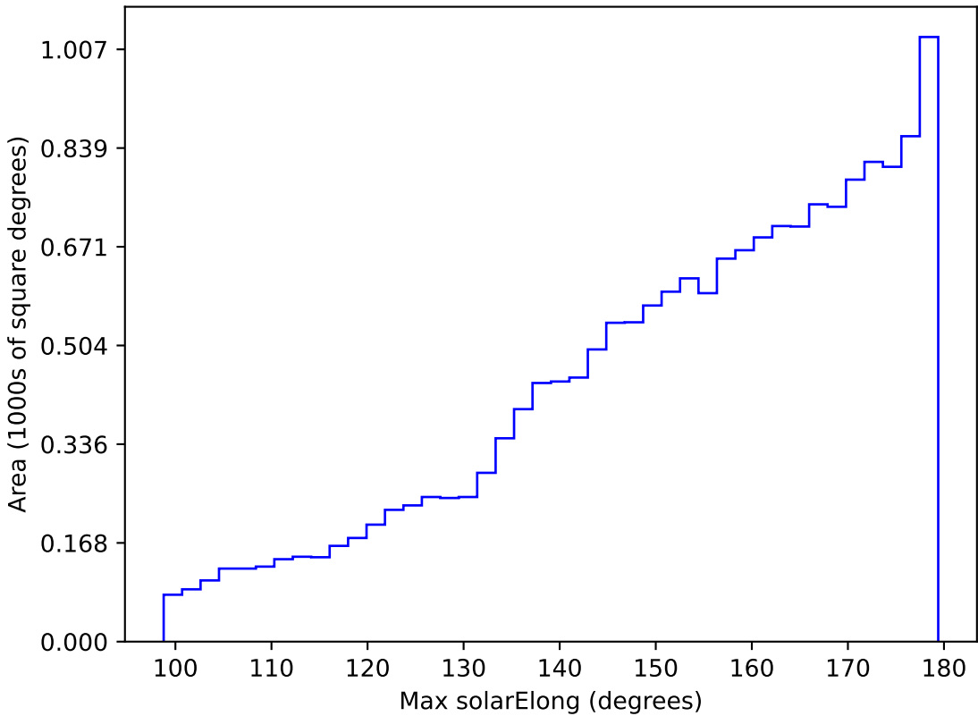
too_elab_r32_d2_ugrizy_v3.4_10yrs WFD r band: Max solarElong
