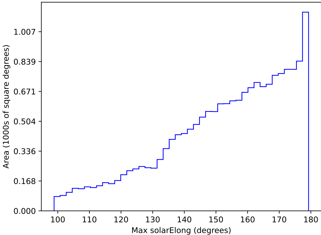
too_elab_r32_d2_ugrizy_v3.4_10yrs WFD i band: Max solarElong
