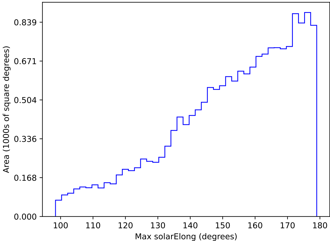
too_elab_r32_d2_ugrizy_v3.4_10yrs WFD g band: Max solarElong
