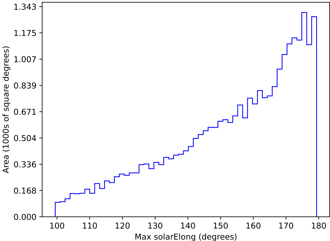
too_elab_r32_d2_ugrizy_v3.4_10yrs All sky z band: Max solarElong
