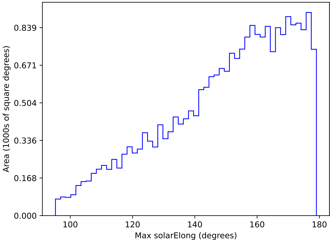
too_elab_r32_d2_ugrizy_v3.4_10yrs All sky u band: Max solarElong
