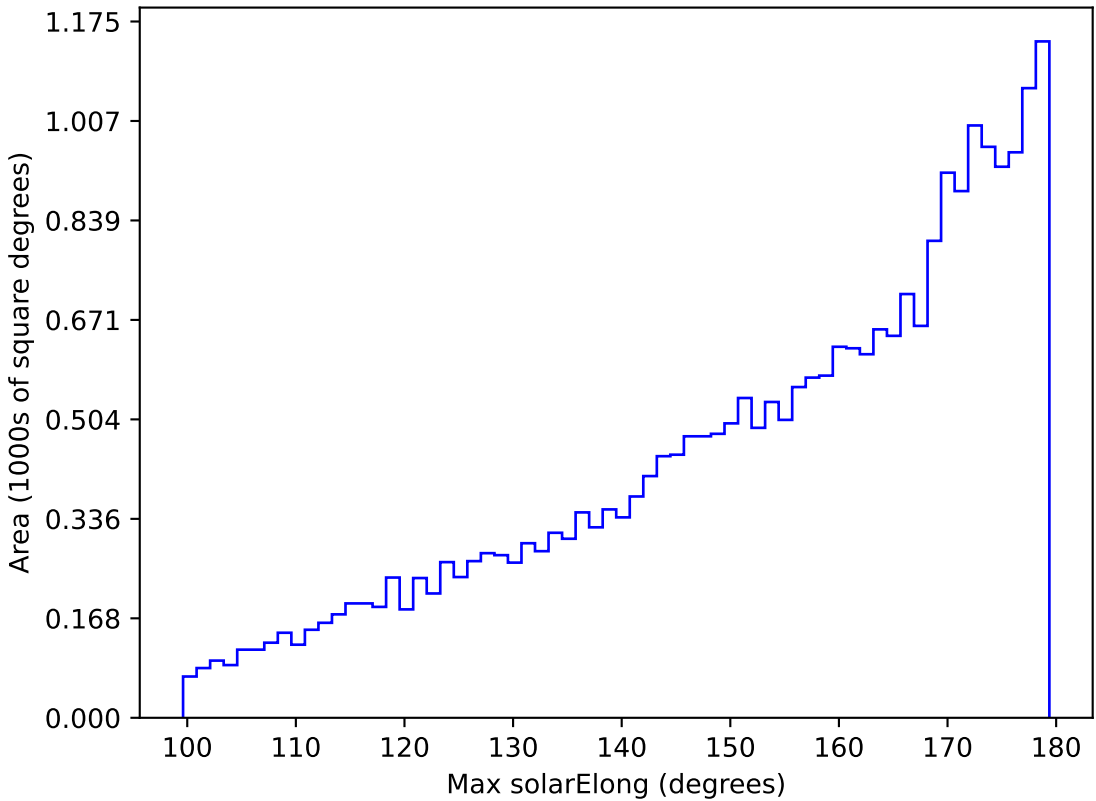
too_elab_r32_d2_ugrizyv3.4_10yrs All sky r band: Max solarElong
