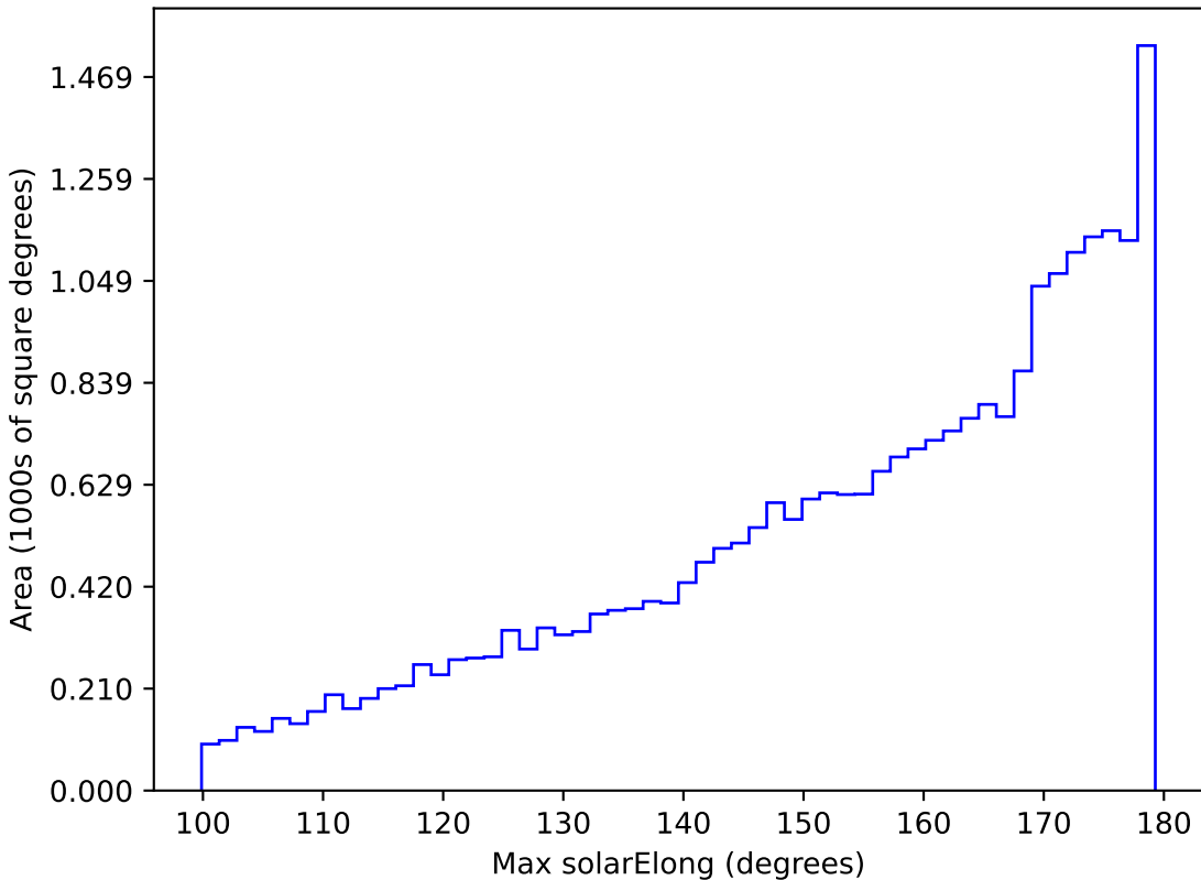
too_elab_r32_d2_ugrizy_v3.4_10yrs All sky i band: Max solarElong
