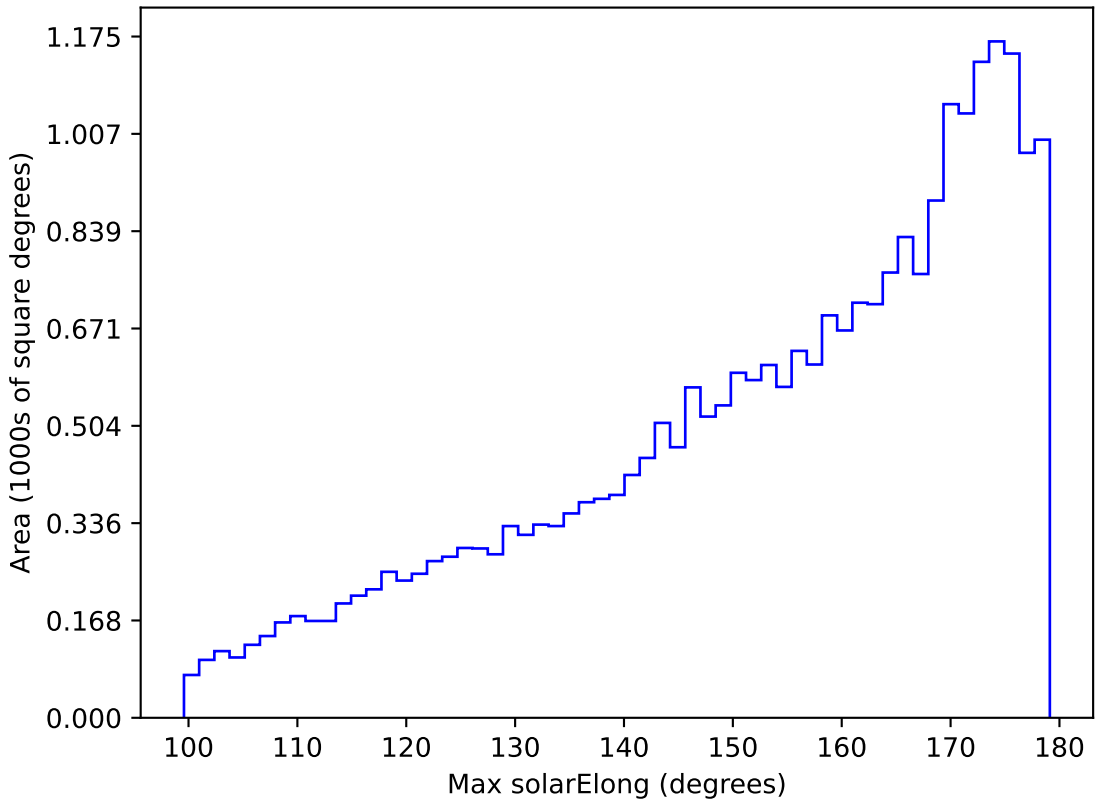
too_elab_r32_d2_ugrizy_v3.4_10yrs All sky g band: Max solarElong
