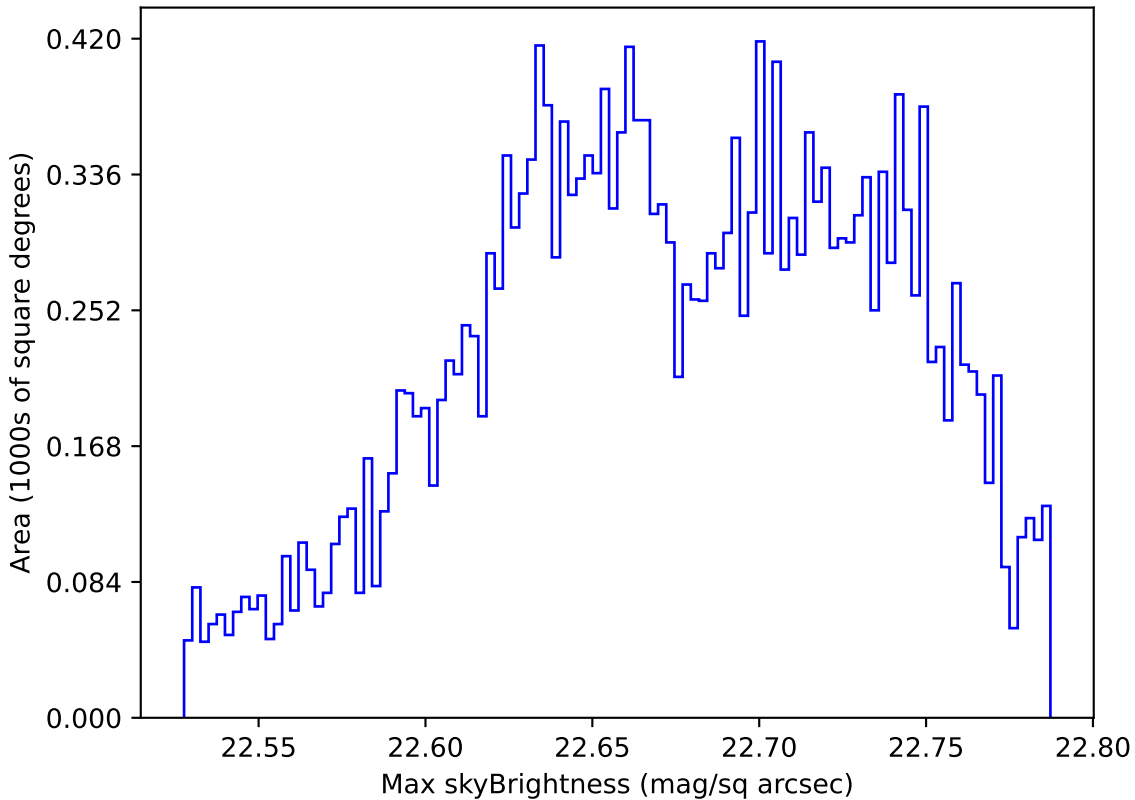
too_elab_r32_d2_ugrizy_v3.4_10yrs Yr 1 u band: Max skyBrightness
