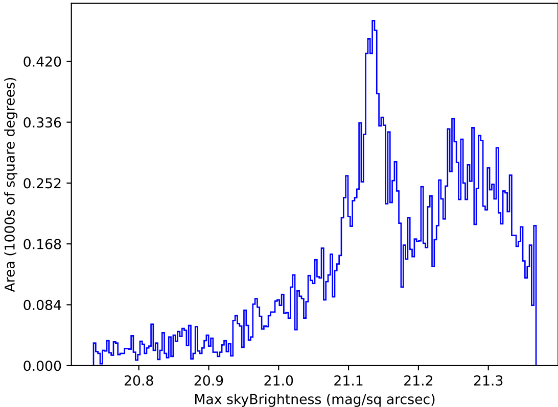
too_elab_r32_d2_ugrizy_v3.4_10yrs Yr 1 r band: Max skyBrightness
