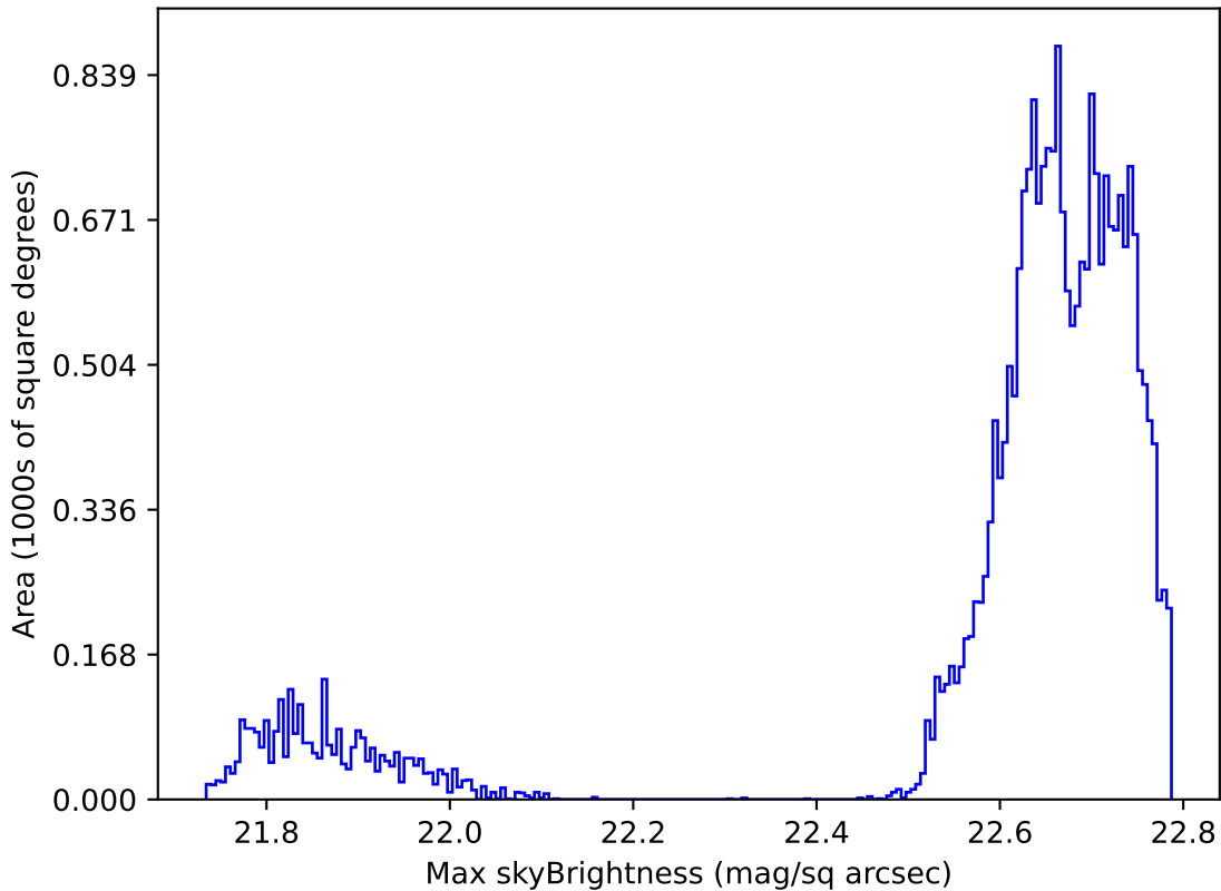
too_elab_r32_d2_ugrizy_v3.4_10yrs Yr 1 all bands: Max skyBrightness
