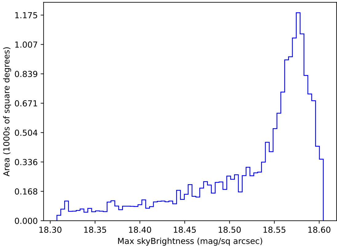
too_elab_r32_d2_ugrizy_v3.4_10yrs WFD y band: Max skyBrightness
