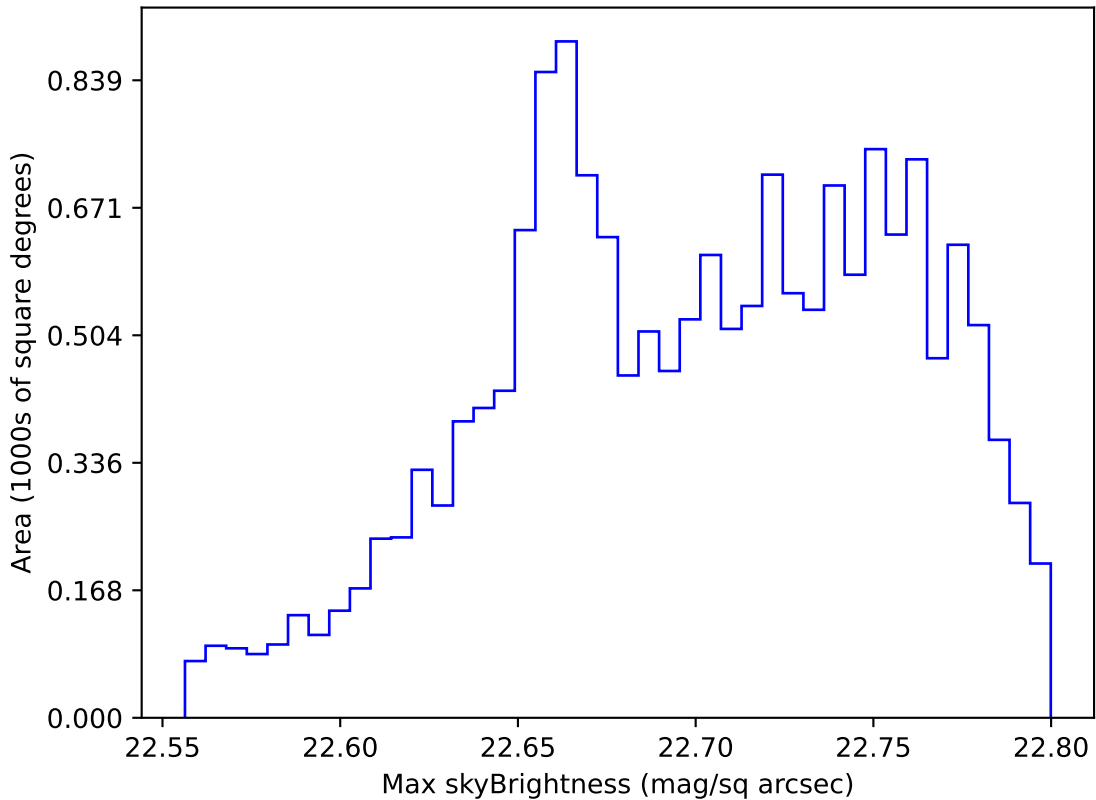
too_elab_r32_d2_ugrizy_v3.4_10yrs WFD u band: Max skyBrightness
