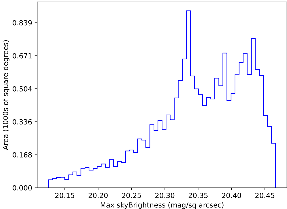
too_elab_r32_d2_ugrizy_v3.4_10yrs WFD i band: Max skyBrightness
