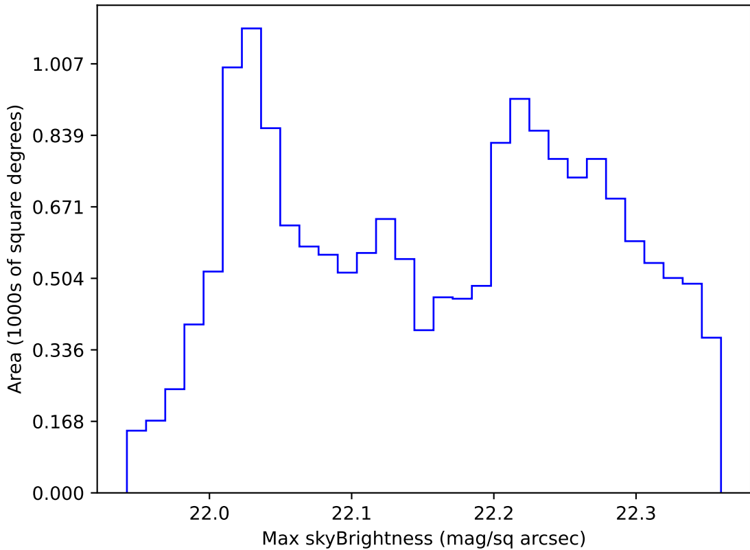
too_elab_r32_d2_ugrizy_v3.4_10yrs WFD g band: Max skyBrightness
