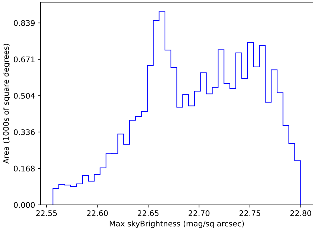
too_elab_r32_d2_ugrizy_v3.4_10yrs WFD all bands: Max skyBrightness
