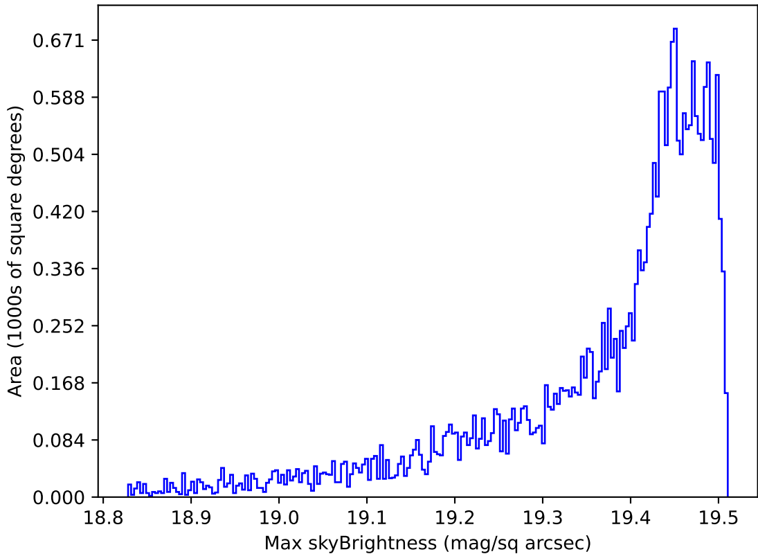
too_elab_r32_d2_ugrizy_v3.4_10yrs All sky z band: Max skyBrightness
