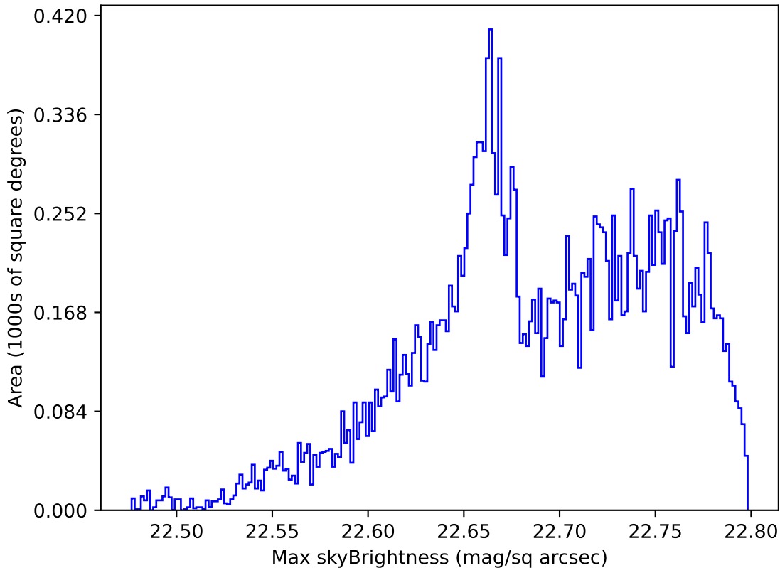
too_elab_r32_d2_ugrizy_v3.4_10yrs All sky u band: Max skyBrightness
