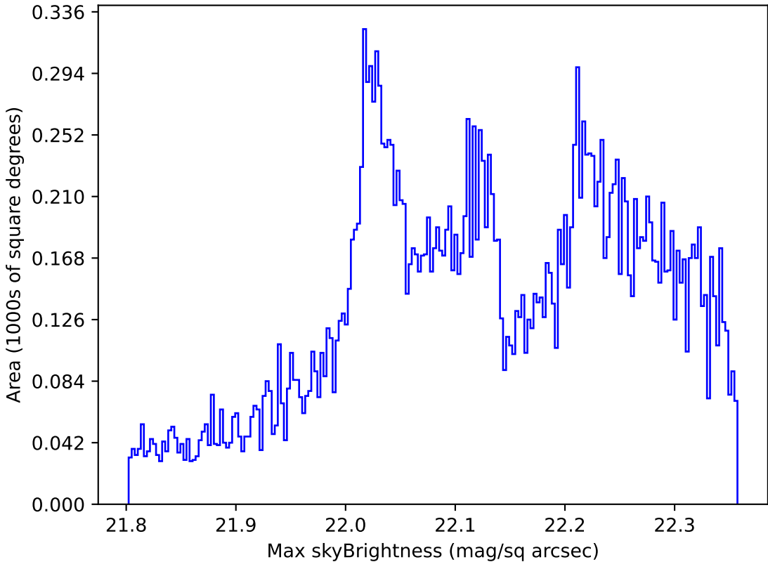
too_elab_r32_d2_ugrizy_v3.4_10yrs All sky g band: Max skyBrightness
