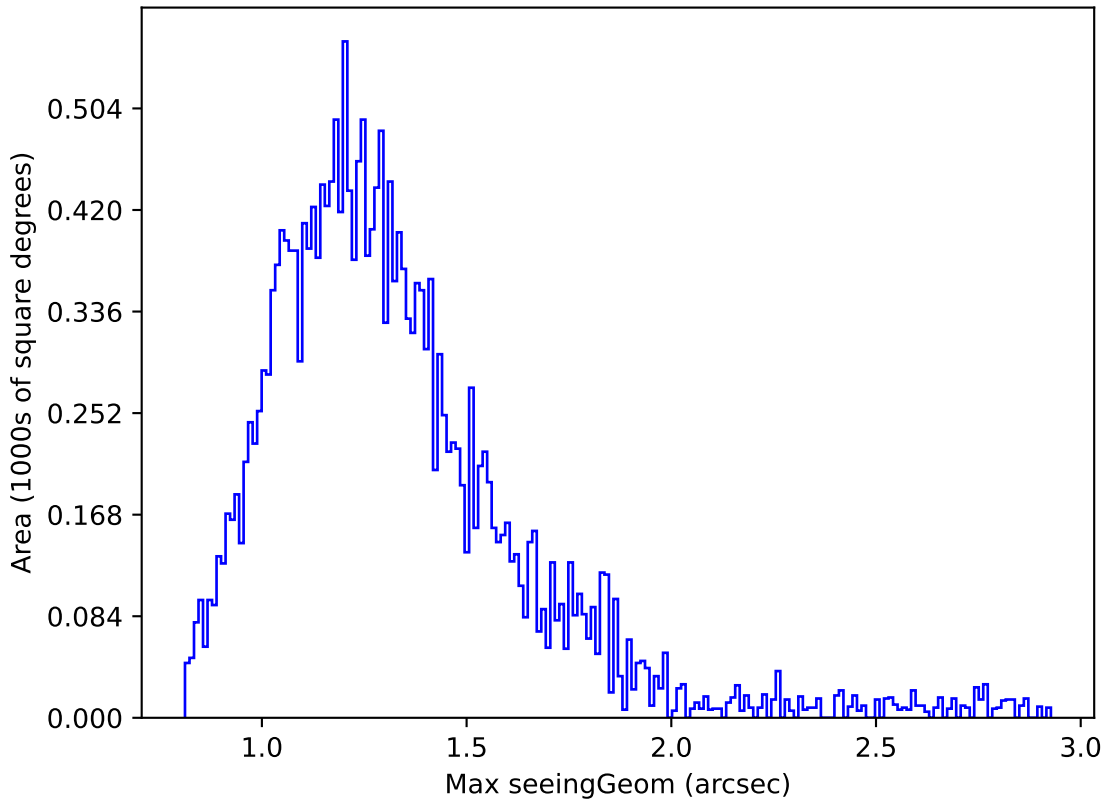
too_elab_r32_d2_ugrizy_v3.4_10yrs Yr 1 u band: Max seeingGeom
