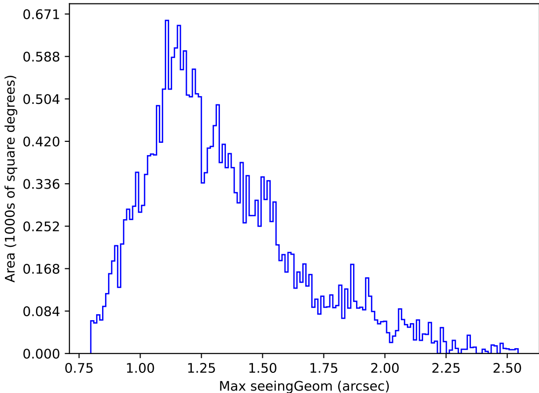
too_elab_r32_d2_ugrizy_v3.4_10yrs Yr 1 i band: Max seeingGeom
