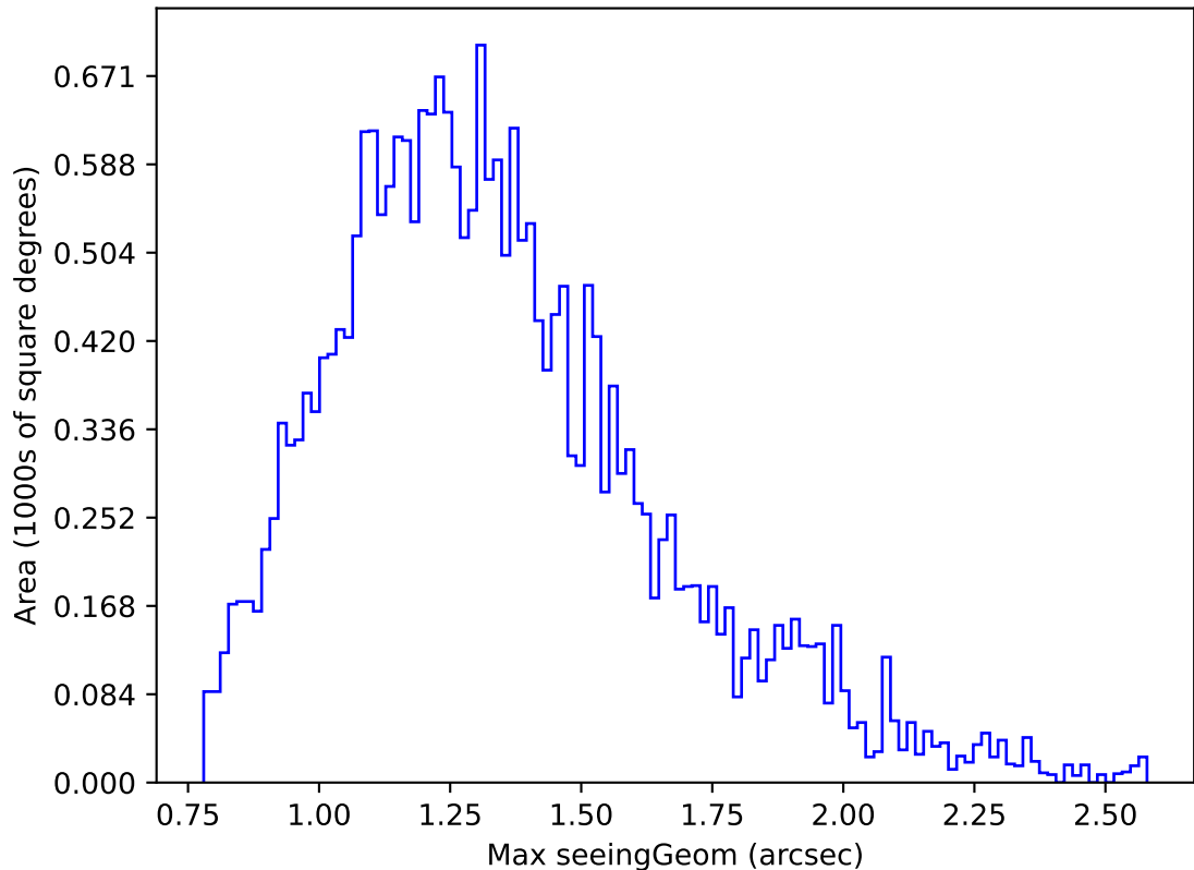
too_elab_r32_d2_ugrizy_v3.4_10yrs Yr 1 g band: Max seeingGeom
