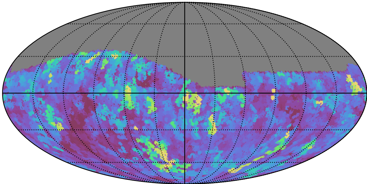
too_elab_r32_d2_ugrizy_v3.4_10yrs Yr 1 z band: Max seeingEff
