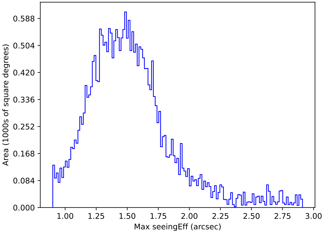
too_elab_r32_d2_ugrizy_v3.4_10yrs Yr 1 z band: Max seeingEff
