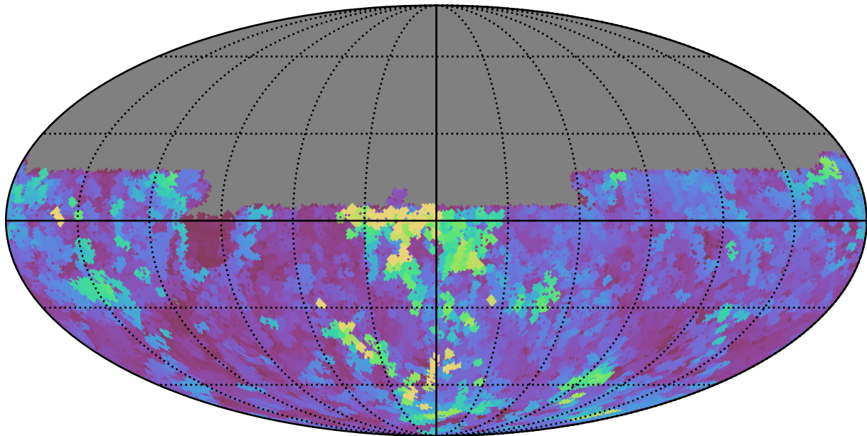
too_elab_r32_d2_ugrizy_v3.4_10yrs Yr 1 y band: Max seeingEff
