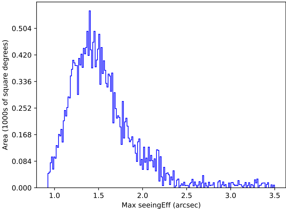
too_elab_r32_d2_ugrizy_v3.4_10yrs Yr 1 u band: Max seeingEff
