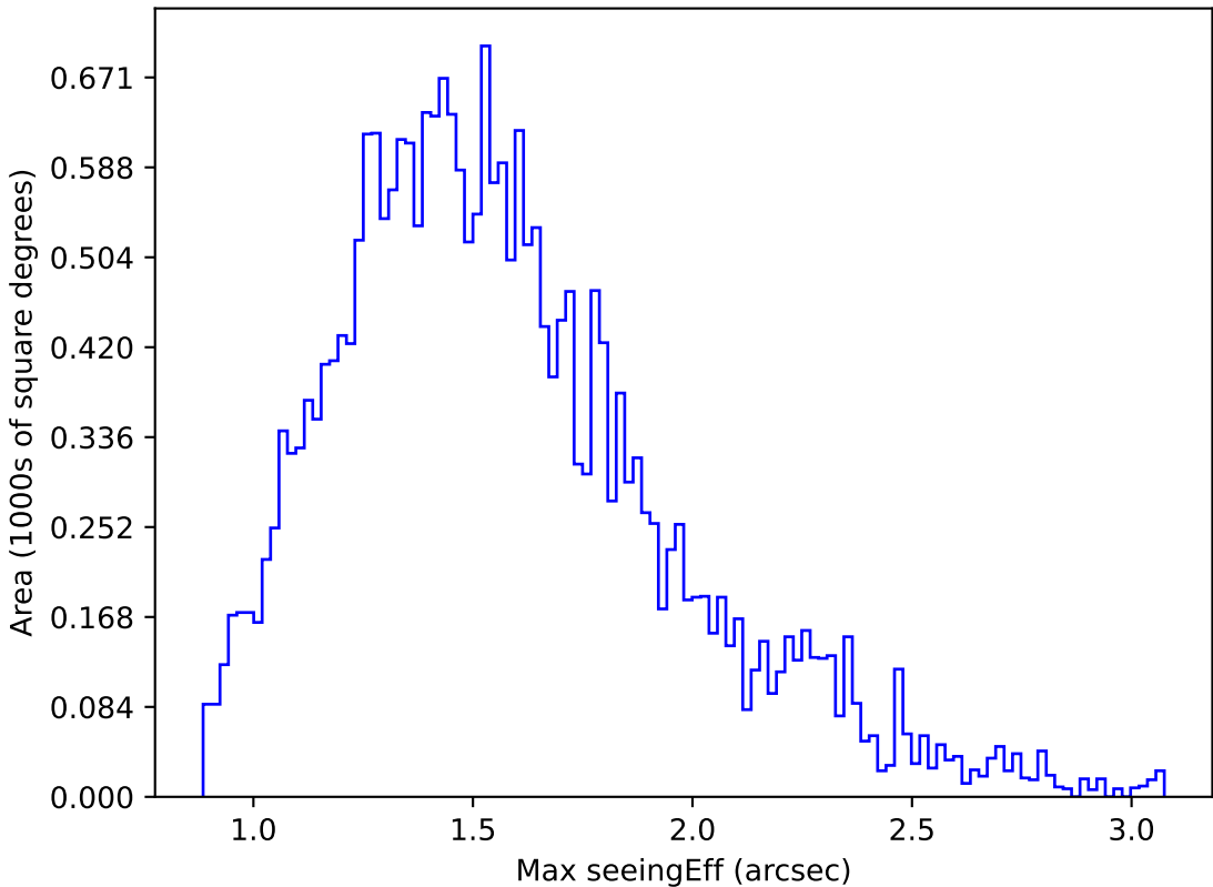
too_elab_r32_d2_ugrizy_v3.4_10yrs Yr 1 g band: Max seeingEff
