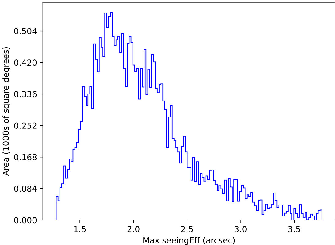
too_elab_r32_d2_ugrizy_v3.4_10yrs Yr 1 all bands: Max seeingEff
