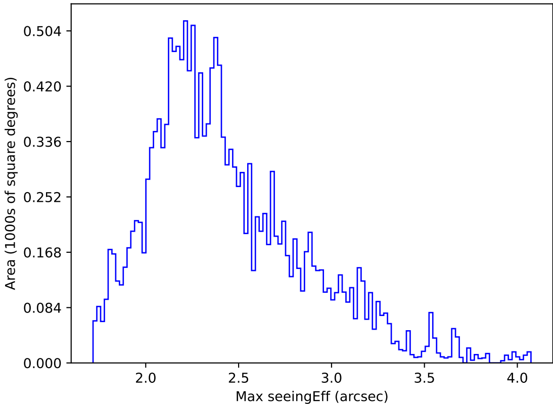
too_elab_r32_d2_ugrizy_v3.4_10yrs WFD u band: Max seeingEff
