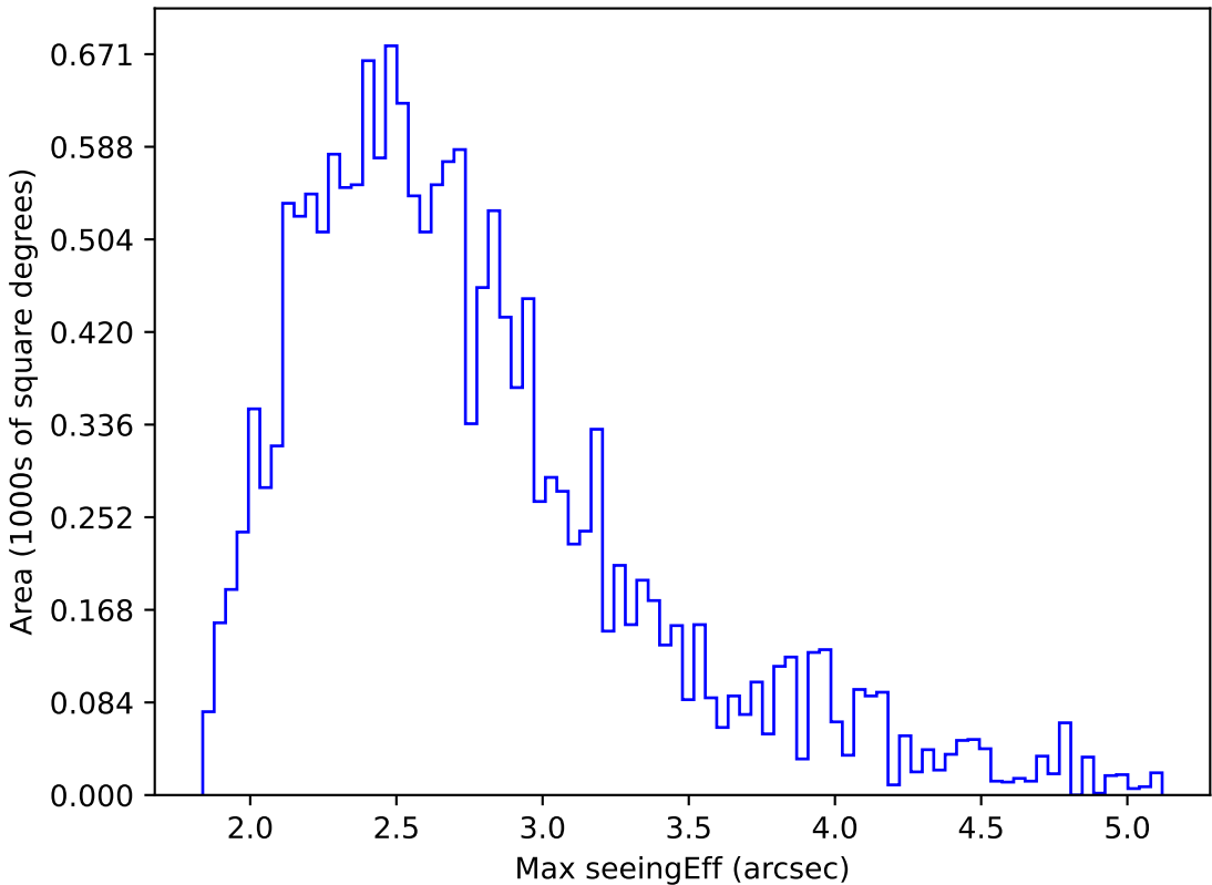
too_elab_r32_d2_ugrizy_v3.4_10yrs WFD r band: Max seeingEff
