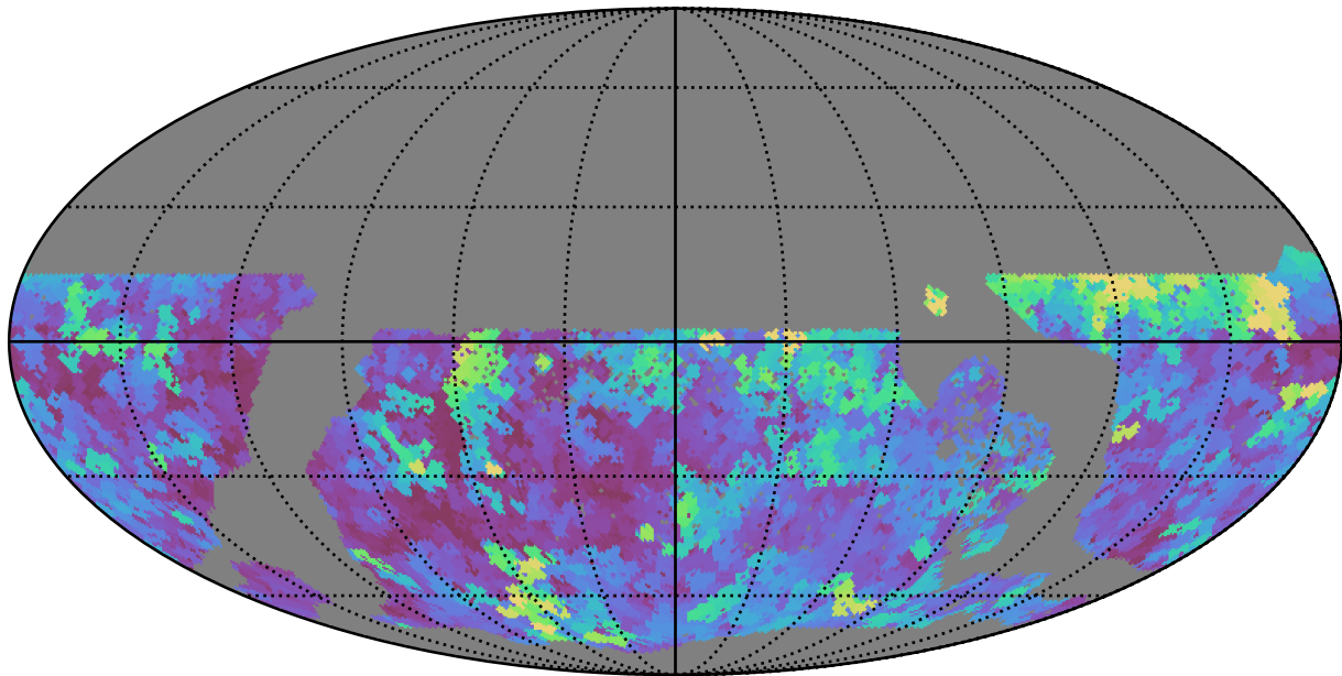
too_elab_r32_d2_ugrizy_v3.4_10yrs WFD g band: Max seeingEff
