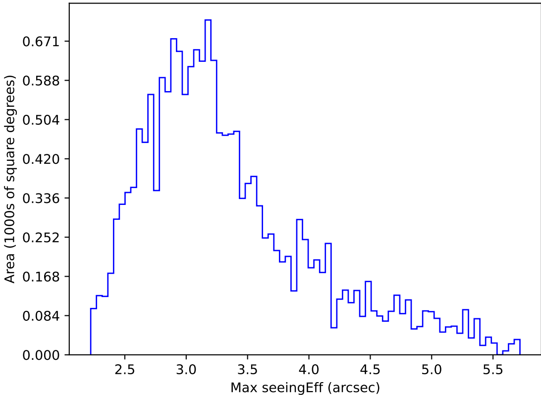
too_elab_r32_d2_ugrizy_v3.4_10yrs WFD all bands: Max seeingEff
