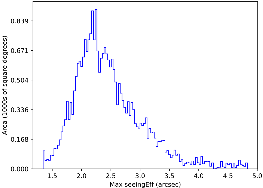
too_elab_r32_d2_ugrizy_v3.4_10yrs All sky z band: Max seeingEff
