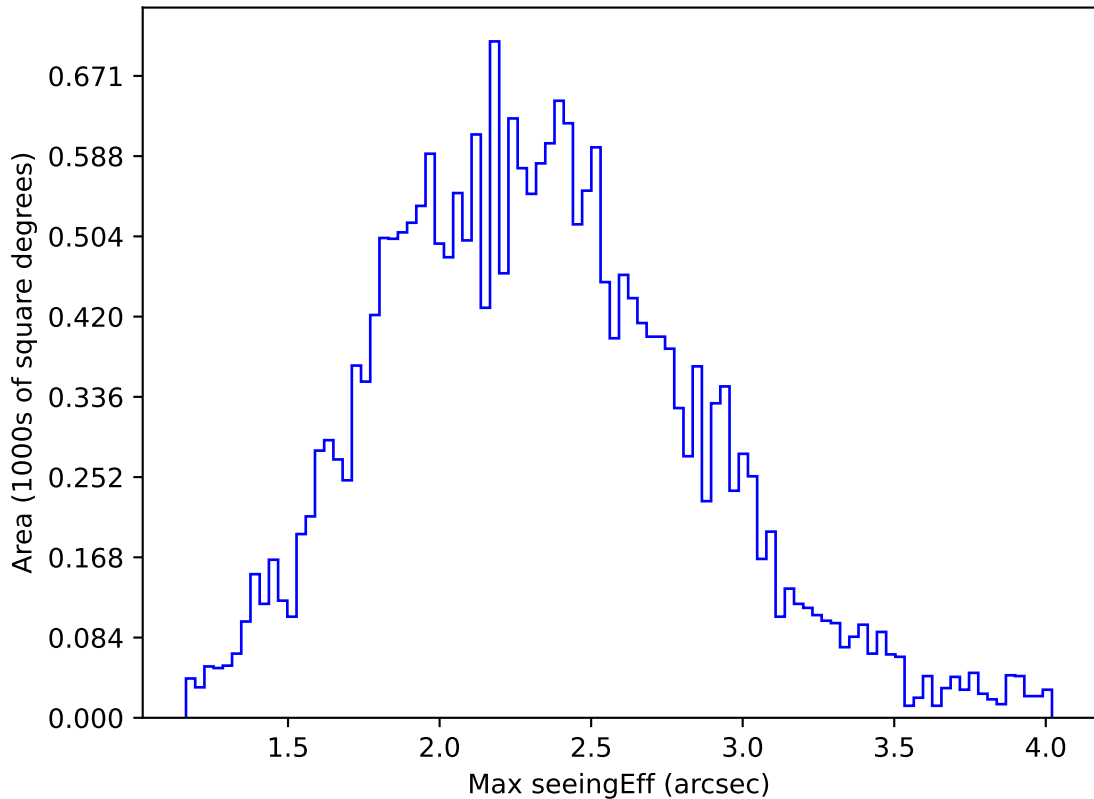
too_elab_r32_d2_ugrizy_v3.4_10yrs All sky y band: Max seeingEff
