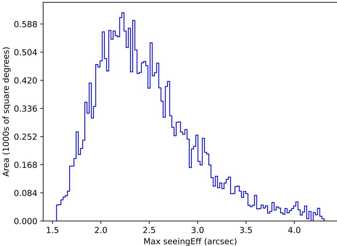
too_elab_r32_d2_ugrizy_v3.4_10yrs All sky g band: Max seeingEff
