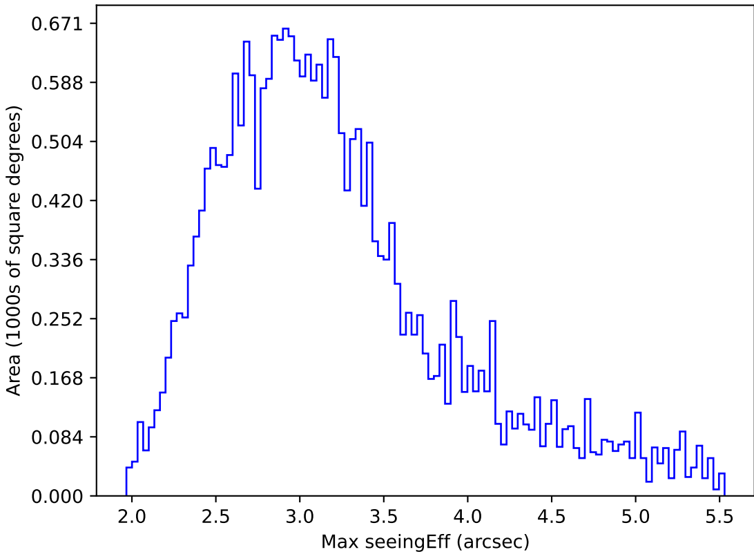
too_elab_r32_d2_ugrizy_v3.4_10yrs All sky all bands: Max seeingEff
