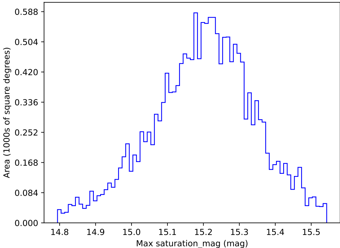
too_elab_r32_d2_ugrizy_v3.4_10yrs WFD z band: Max saturation_mag
