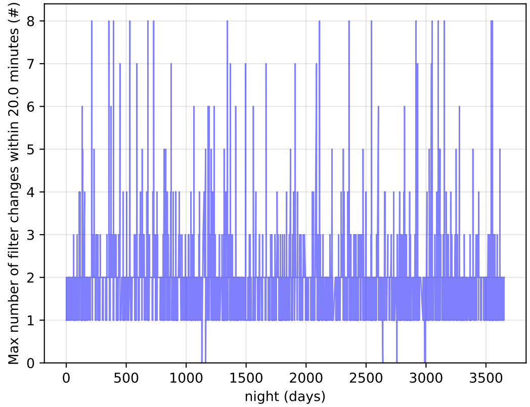
too_elab_r32_d2_ugrizyv3.4_10yrs Per Night: Max number of filter changes within 20.0 minutes
