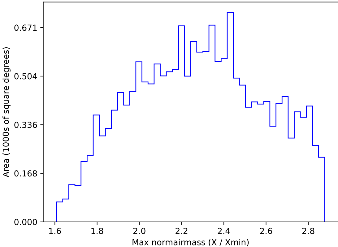
too_elab_r32_d2_ugrizy_v3.4_10yrs WFD z band: Max normairmass
