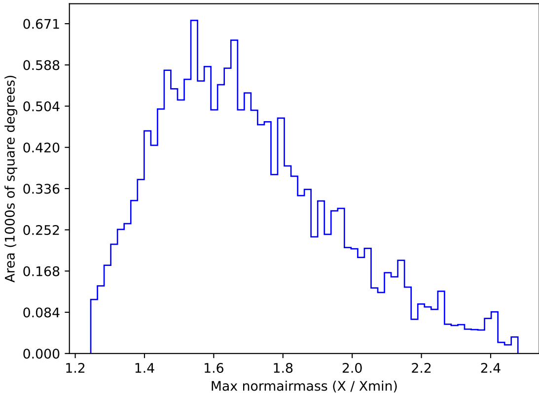
too_elab_r32_d2_ugrizy_v3.4_10yrs WFD u band: Max normairmass
