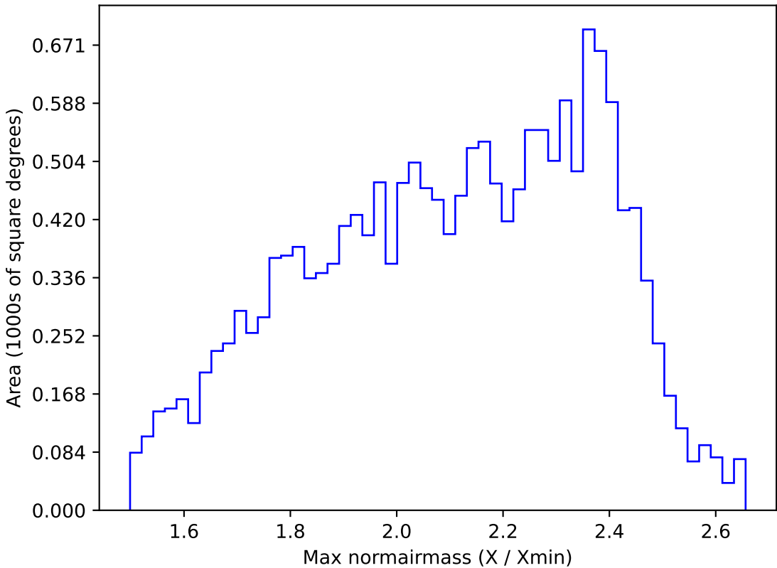
too_elab_r32_d2_ugrizy_v3.4_10yrs WFD r band: Max normairmass
