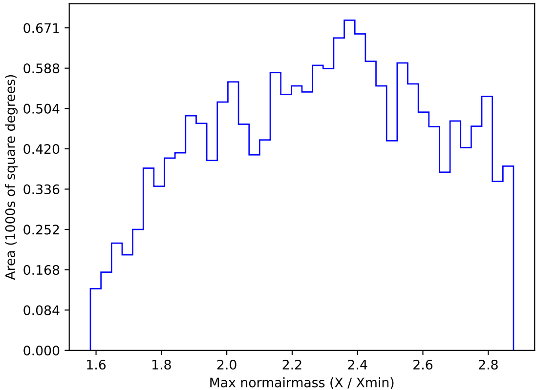
too_elab_r32_d2_ugrizy_v3.4_10yrs WFD i band: Max normairmass
