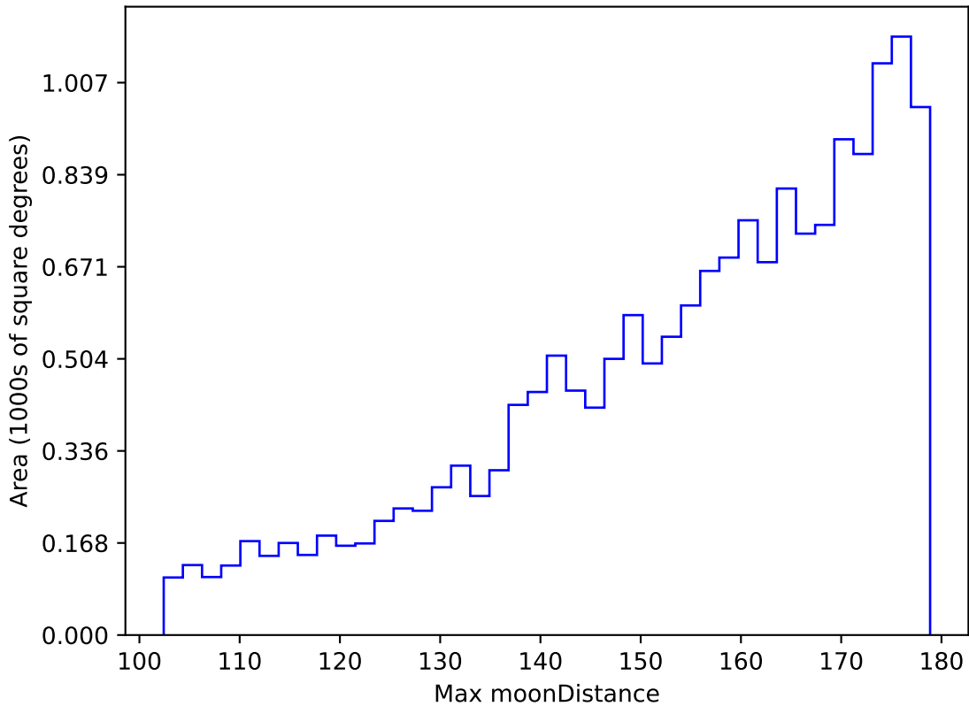
too_elab_r32_d2_ugrizy_v3.4_10yrs WFD z band: Max moonDistance
