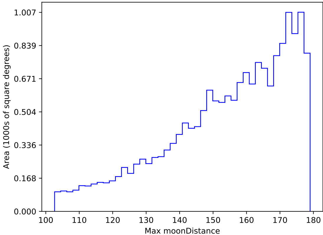
too_elab_r32_d2_ugrizy_v3.4_10yrs WFD u band: Max moonDistance
