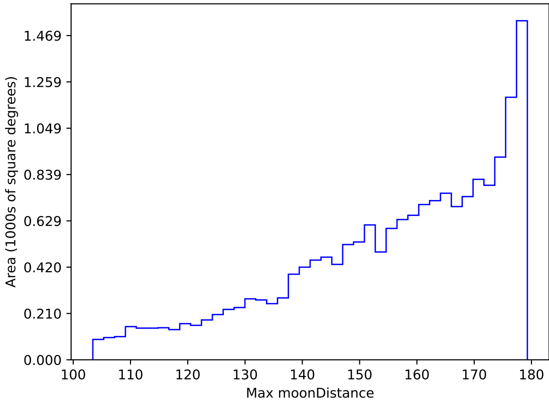
too_elab_r32_d2_ugrizy_v3.4_10yrs WFD r band: Max moonDistance
