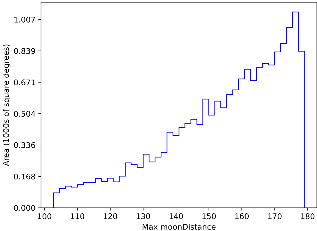
too_elab_r32_d2_ugrizy_v3.4_10yrs WFD g band: Max moonDistance
