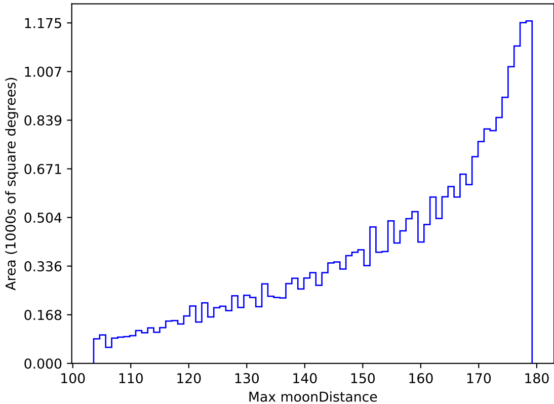
too_elab_r32_d2_ugrizy_v3.4_10yrs All sky r band: Max moonDistance
